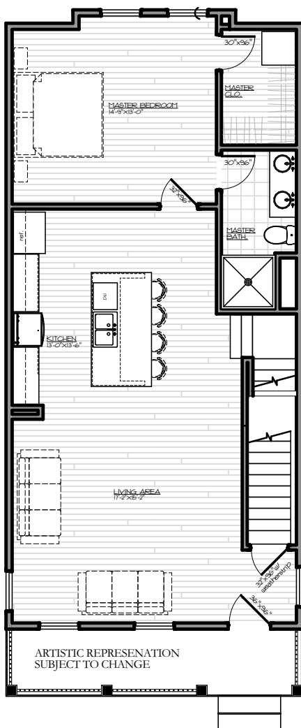
FIRST FLOOR 1002 Square Feet
