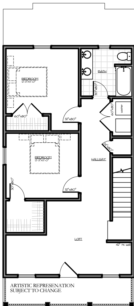
SECOND FLOOR 854 Square Feet
