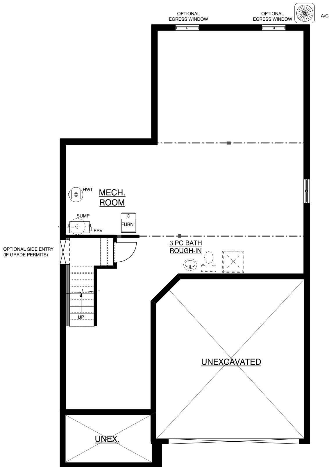
Standard Unfinished Basement
