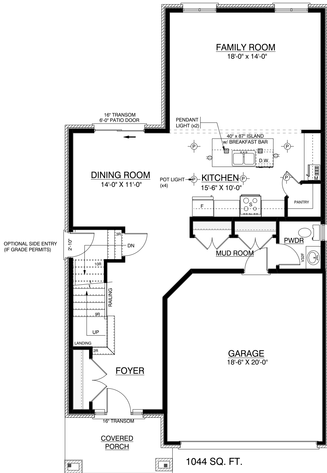
Main Floor Kitchen Layout 'A'
