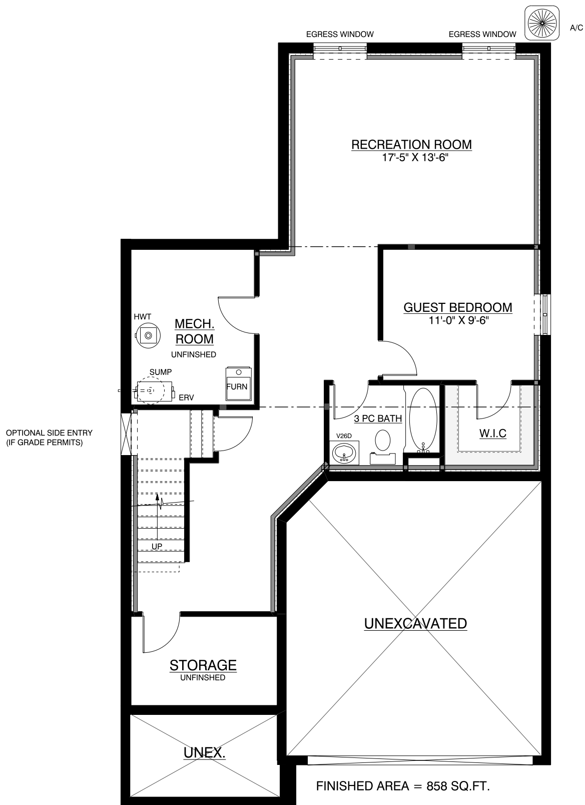
'Optional' Finished Basement
