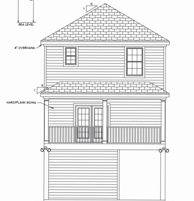
REAR ELEVATION
