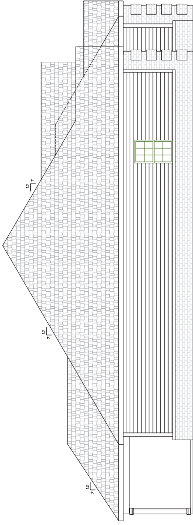
3 LEFT ELEVATION AS-2 SCALE: 1/4" = 1'-0"
