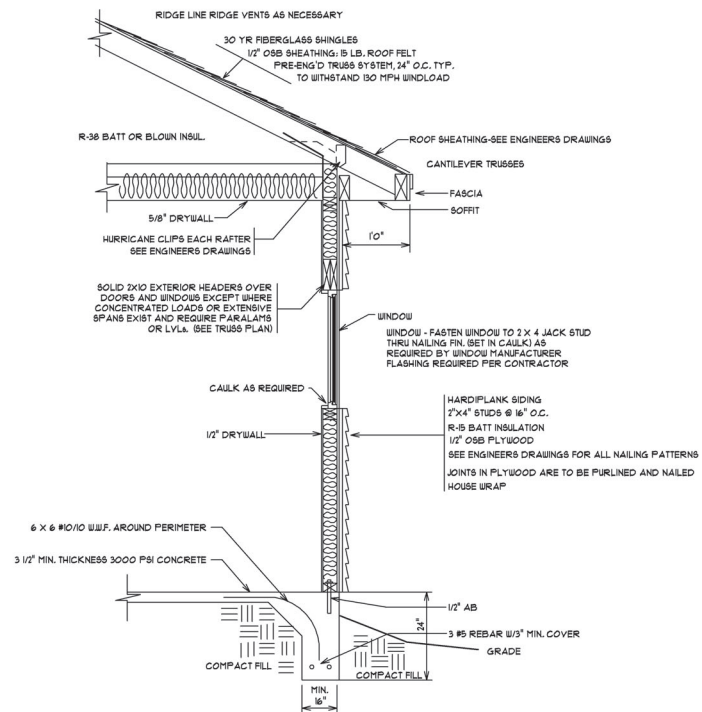
CROSS SECTION DETAIL MONOLITHIC SLAB-HARDIPLANK SIDING NOT TO SCALE
