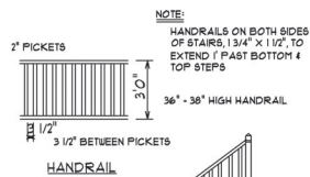
HANDRAIL
