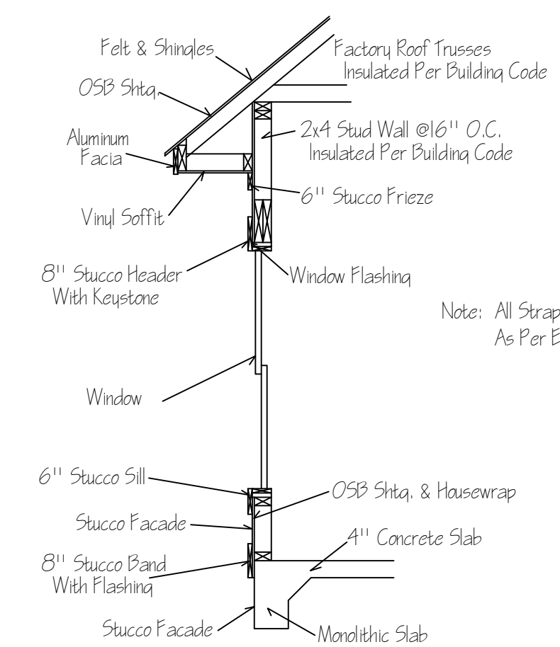
STUCCO SECTION DETAIL NTS
