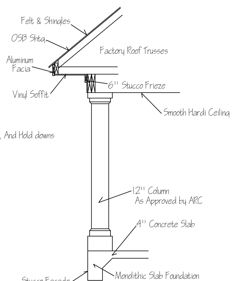
PORCH SECTION DETAIL NTS
