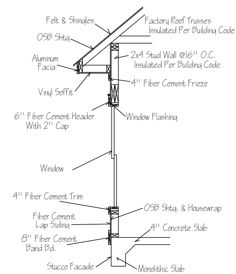
SIDING SECTION DETAIL NTS
