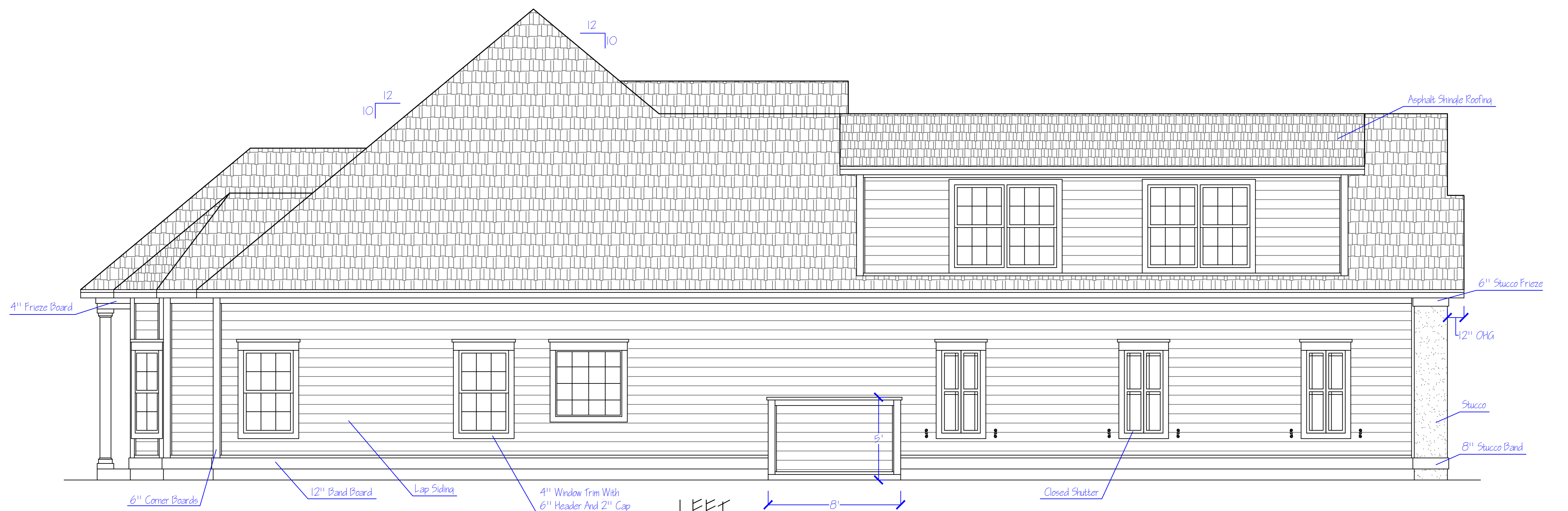
LEFT 1/4 INCH SCALE
