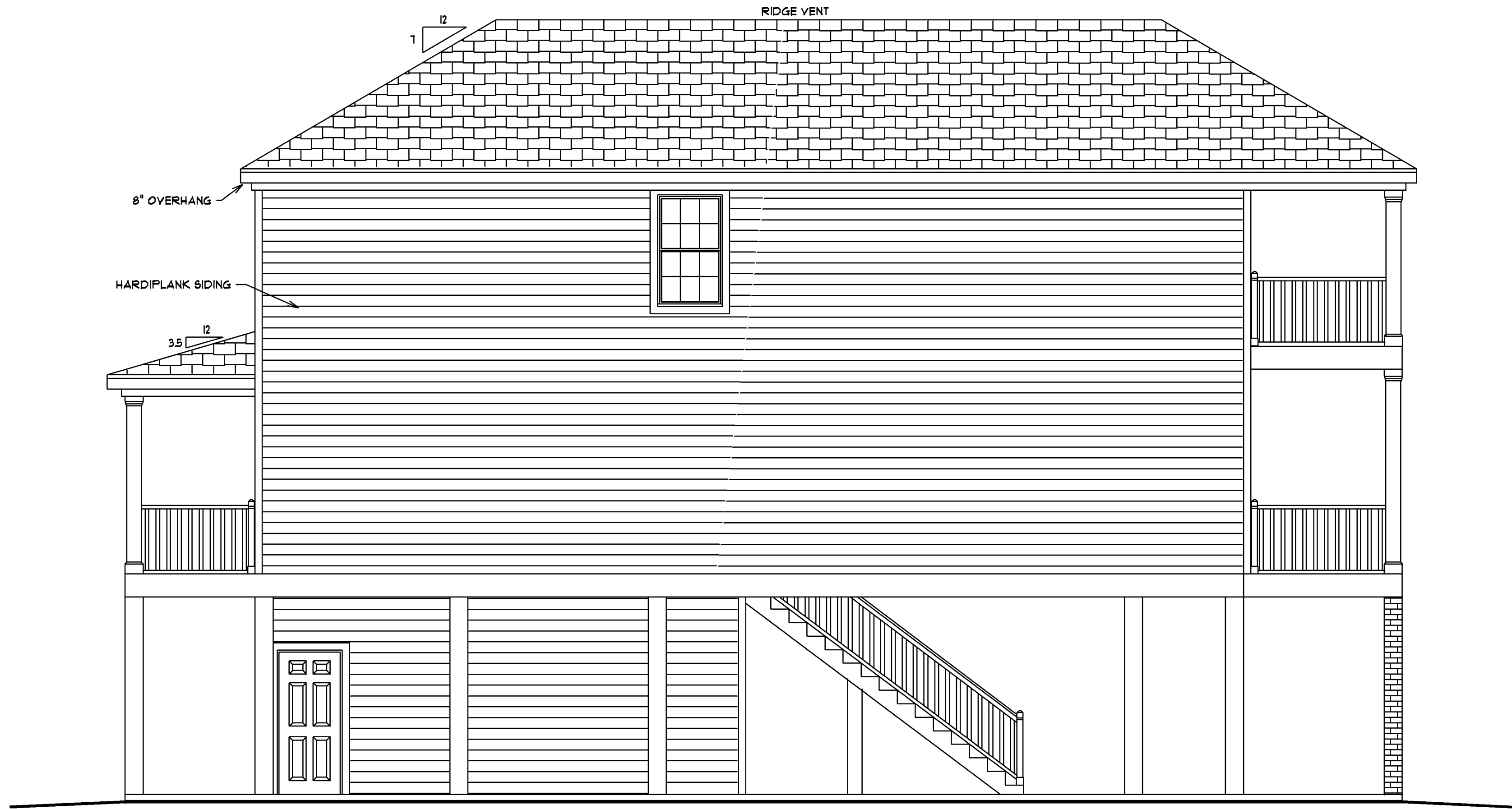
LEFT ELEVATION
