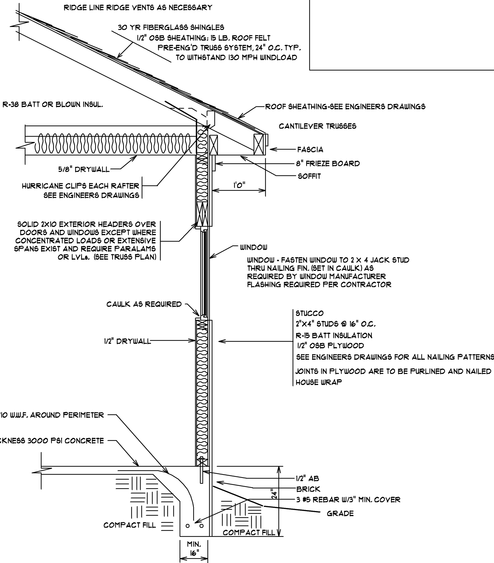
CROSS SECTION DETAIL MONOLITHIC SLAB-STUCCO NOT TO SCALE
