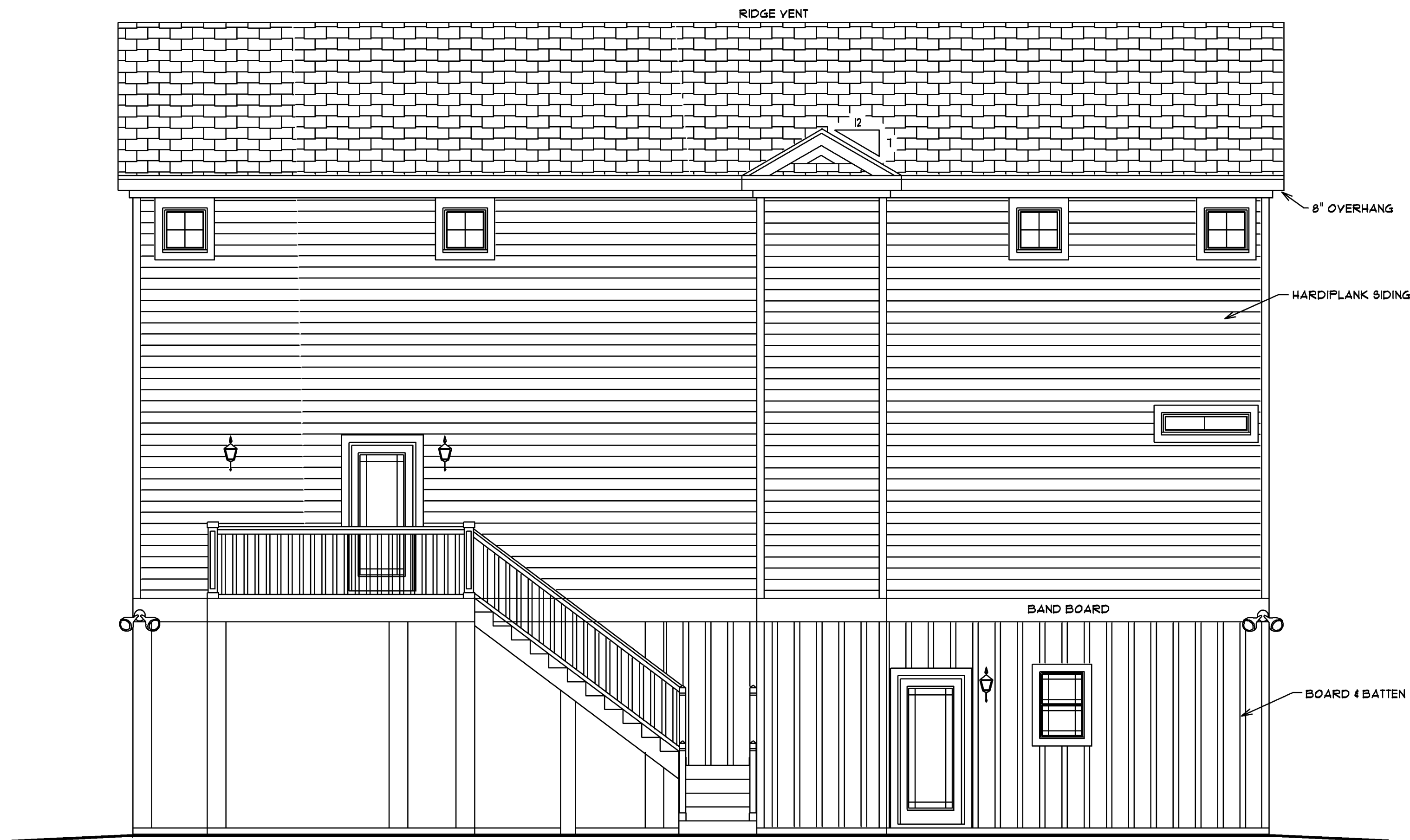
REAR ELEVATION
