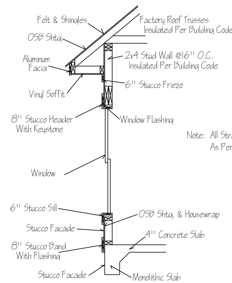
STUCCO SECTION DETAIL NTS
