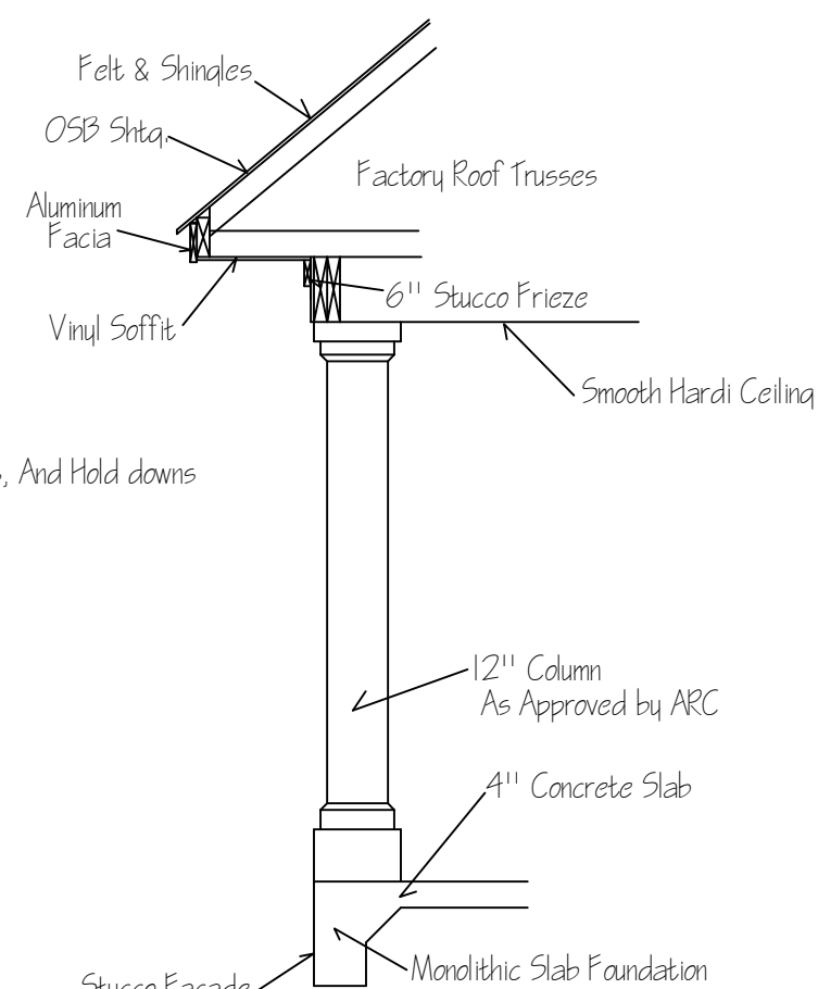
PORCH SECTION DETAIL NTS
