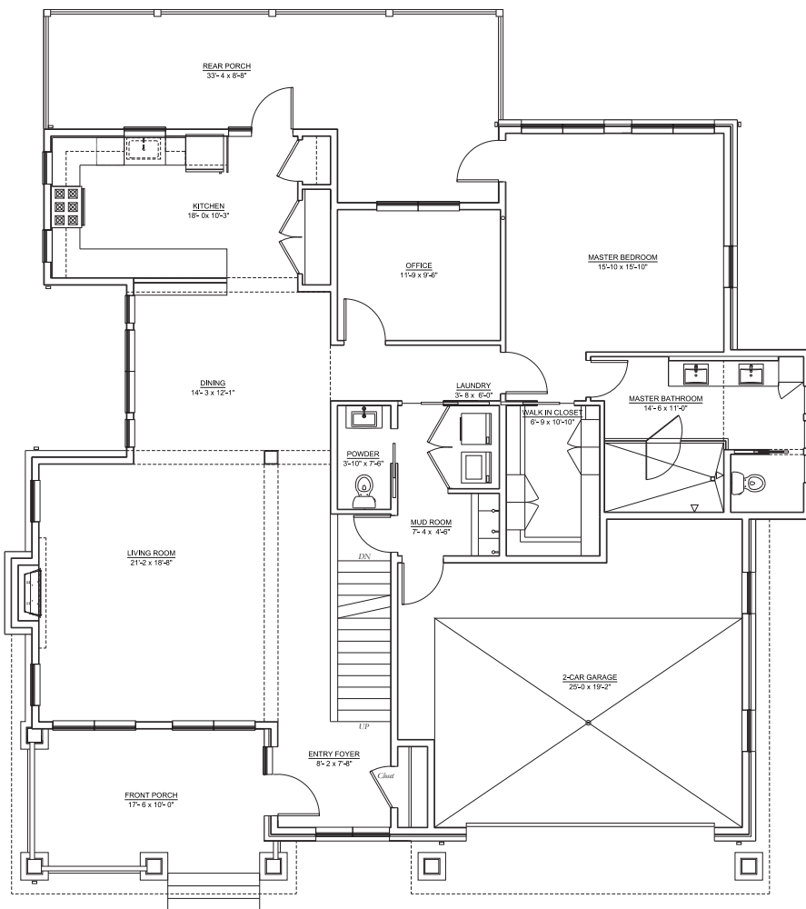
FIRST FLOOR
