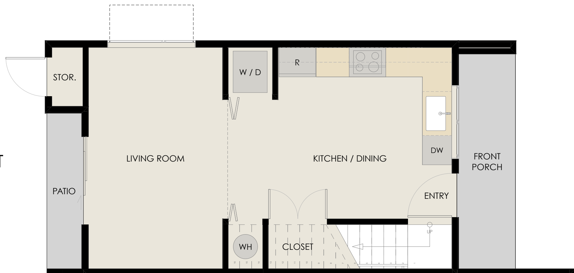
LOT 1 MODEL 'B' STUDIO LOFT 599 SF
