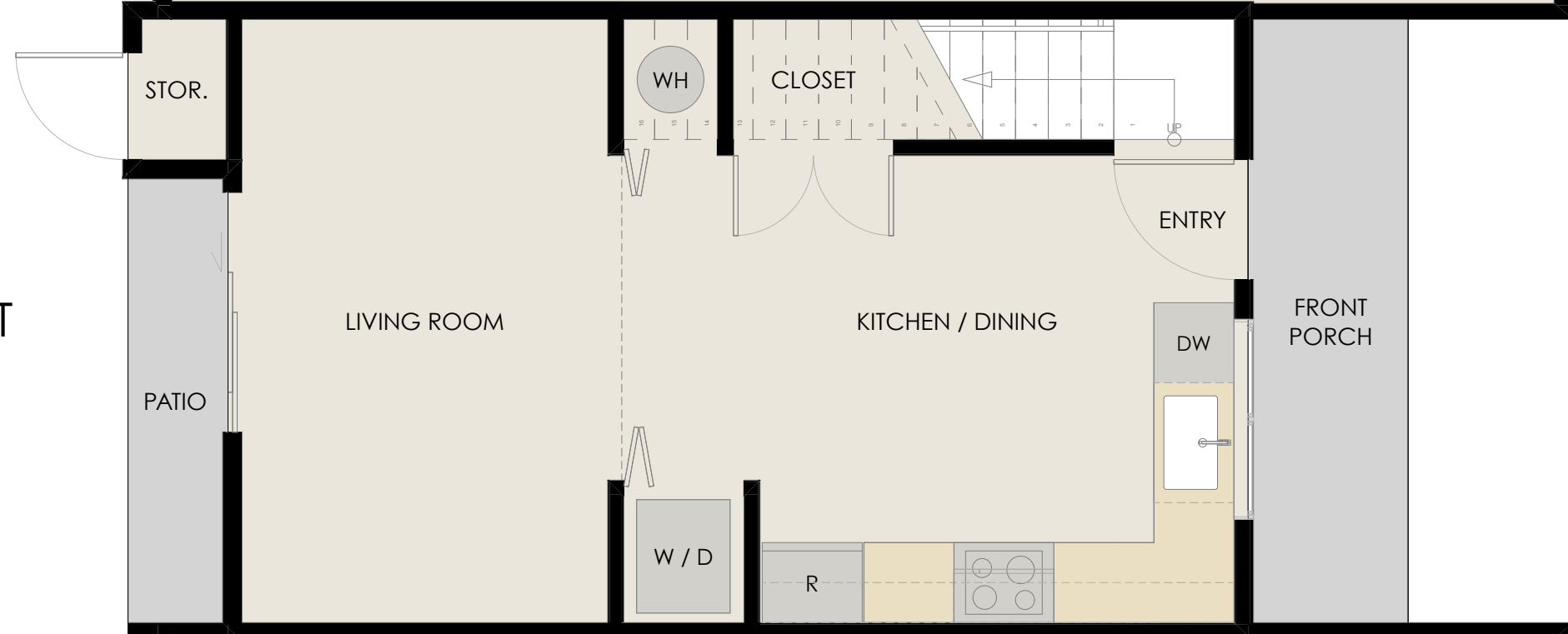
LOT 5 MODEL 'A' STUDIO LOFT 599 SF
